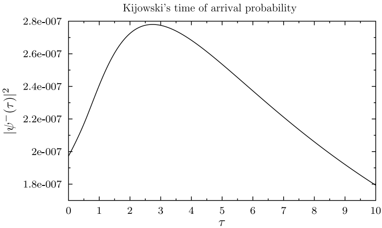
Fig. 4. Left mover time of arrival distribution.
