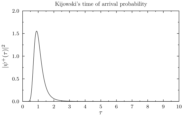
Fig. 3. Right mover time of arrival distribution.
