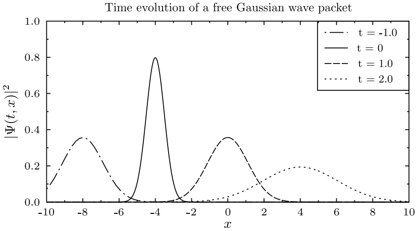
Fig. 1. Free motion of the Gaussian wave packet \Psi(t, x) .
