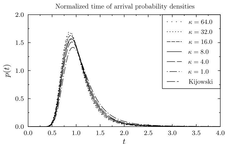
Fig. 7. Normalized arrival times for different \kappa .
