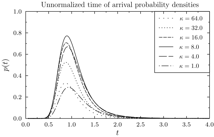
Fig. 5. Time of arrival according to EEQT.
