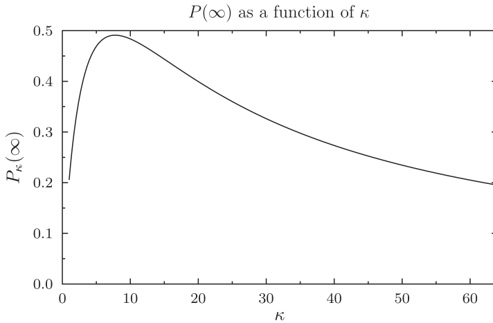
Fig. 6. Total probability of detection.
