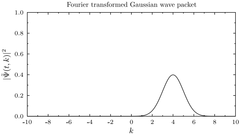
Fig. 2. Fourier transformed evolution \tilde{\Psi}(t, k) .
