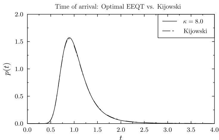
Fig. 8. Is the difference between the two curves only due to the numerical approximation?
